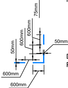
Diagram 1028.4 Parking bay line markings
