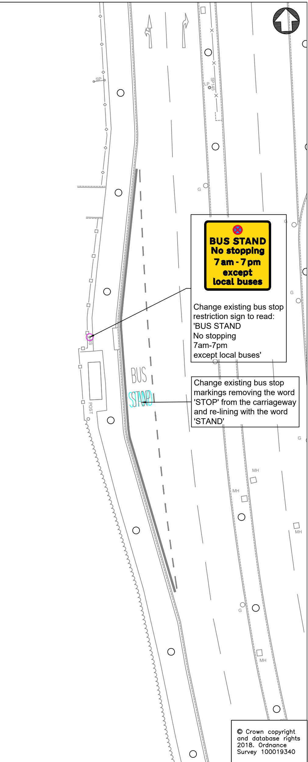
William Frost Way Bus Stop proposed layout @ 1:250
